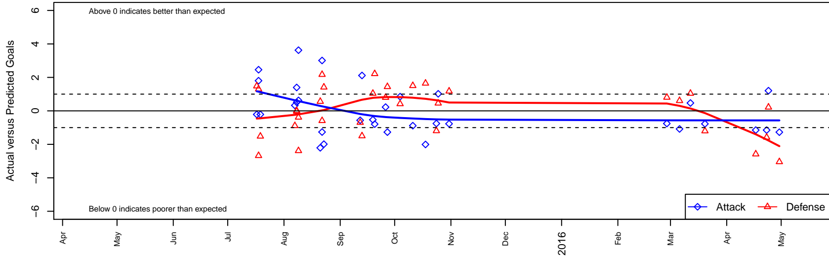
CYSA Timber Barons Green G02 Dots are actual minus expected GF (blue circles) and GA (red triangles). Blue line is smoothed change in attack strength. Red is smoothed change in defense strength.
